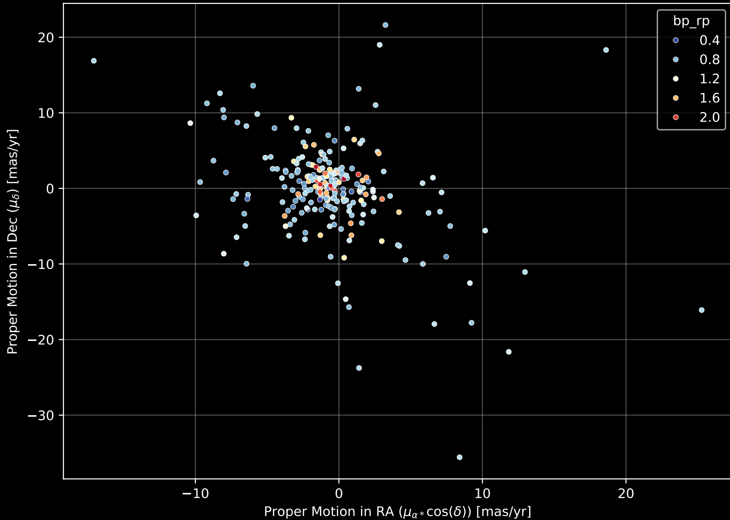
GALAH DR4 Field: [8824] Proper Motion Diagram (n= 246)
