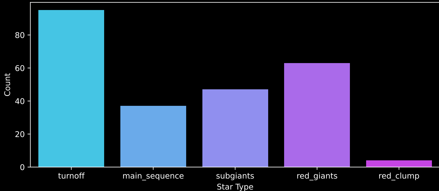
GALAH DR4 Field: [8824] Count plot of Star Type
