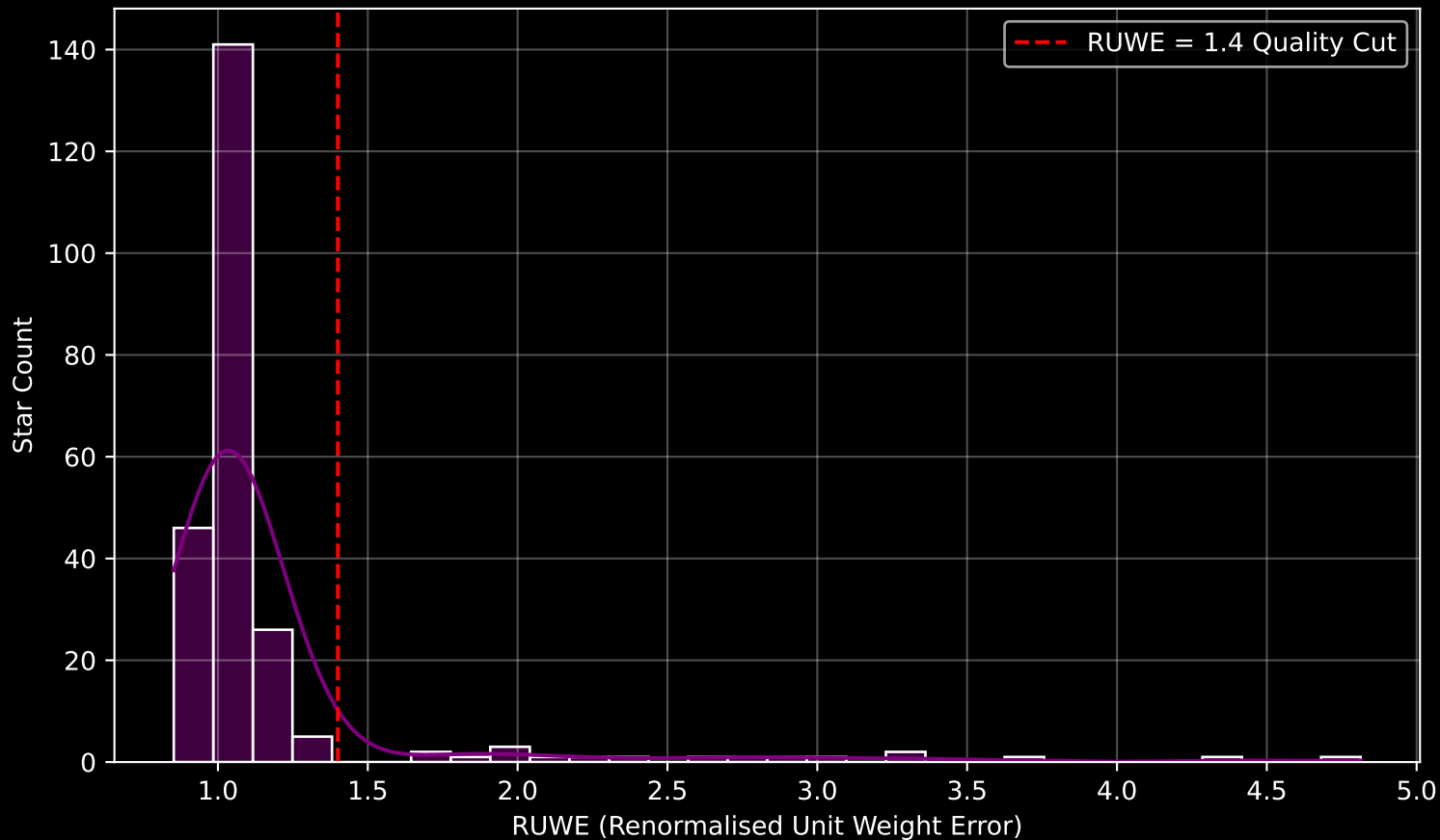
GALAH DR4 Field [8824] RUWE Distribution (n= 236)
